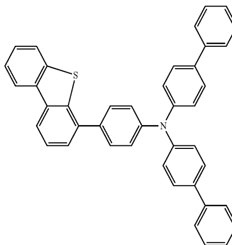
Chemical Formula 1-6
