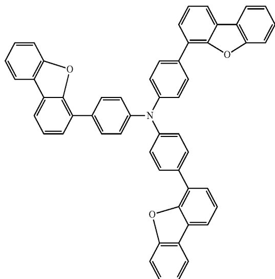
Chemical Formula 1-2
