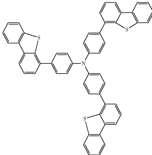
Chemical Formula 1-5
