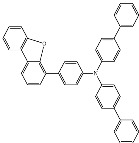
Chemical Formula 1-3
